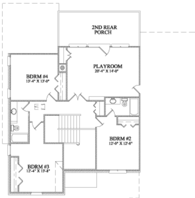
Second Floor - 1,213 sq. ft.
